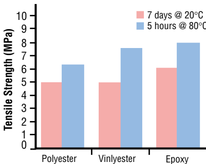
Comparative Tensile Strength of Resins
