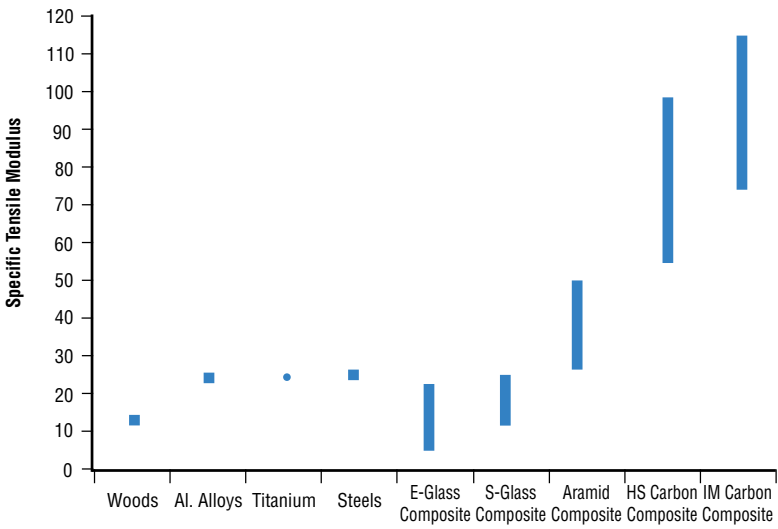
Specific Tensile Modulus of Common Structural Materials
