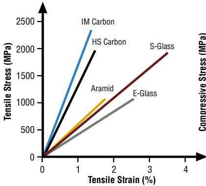
Tensile Properties of U/D Prepreg Laminate Fig. 27
