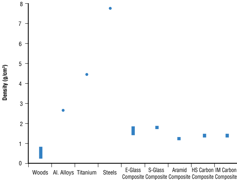
Densities of Common Structural Materials
