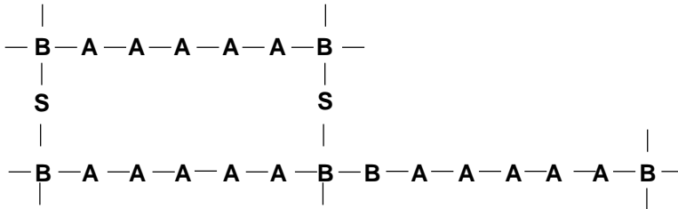
Schematic Representation of Vinyl ester Resin (Cured)
