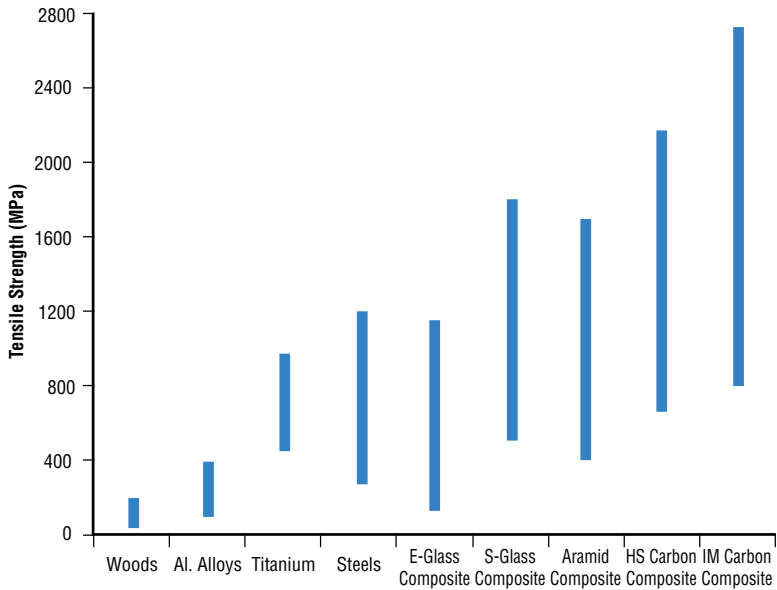
Tensile Strength of Common Structural Materials
