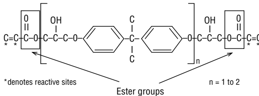
Idealised Chemical Structure of a Typical Epoxy Based Vinylester
