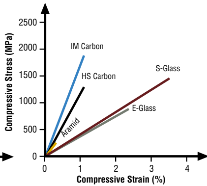
Compressive Properties of U/D Prepreg Laminates Fig. 28
