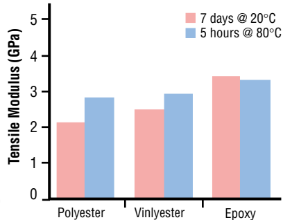
Comparative Stiffness of Resins
