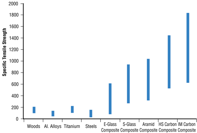
Specific Tensile Strength of Common Structural Materials
