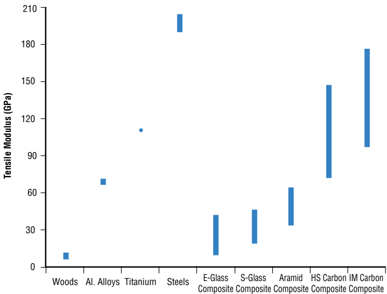
Tensile Modulus of Common Structural Materials
